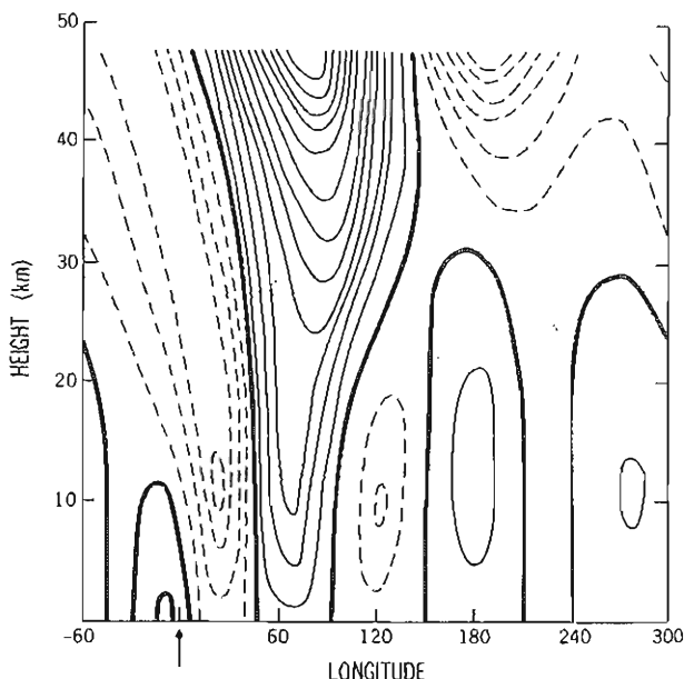
Fig. 6.18. The solution to Eqs. (6.21)–(6.22) with h_T(x) = \delta(x) \sin(ly) . The arrow marks the location of the source. Solid lines are positive contours and dotted lines negative.
