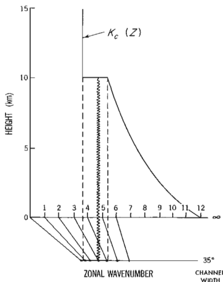
Fig. 6.15. The critical total wavenumber, K_c(z) , dividing the locally propagating ( K < K_c ) from the locally evanescent solutions ( K > K_c ). The zonal wavenumber which yields this total wavenumber if the meridional structure is a half wavelength sine wave in a channel of width 35^\circ is also indicated. The wavy line marks the wavenumber of the stationary external Rossby wave.
