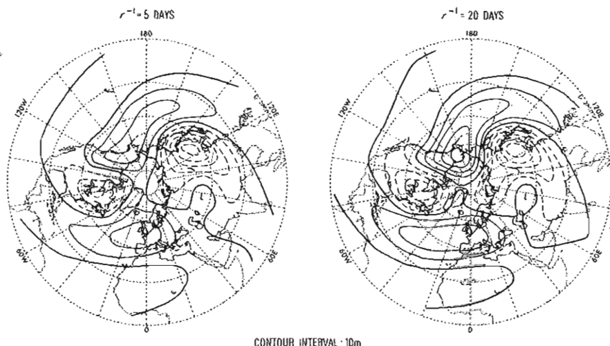
Fig. 6.8. As in Fig. 6.7, but for the height response, f\psi/g .
