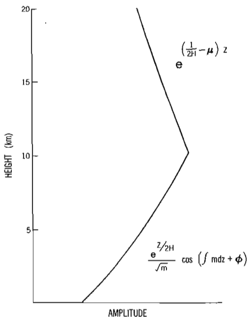
Fig. 6.17. The vertical structure of the external Rossby wave as computed numerically. The expressions alongside the curve are the WKB approximations to this structure.
