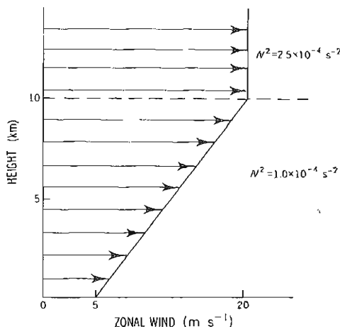
Fig. 6.14. Zonal wind profile and static stabilities used for calculations described in Figs. 6.15–6.18.
