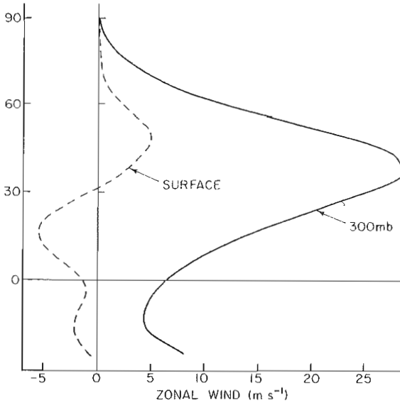
Fig. 6.6. The upper tropospheric and surface winds in the Northern Hemisphere used for [u] and [u_s] in Eqn. (6.12), taken from the 'no-mountain' model described in Section 6.6.
