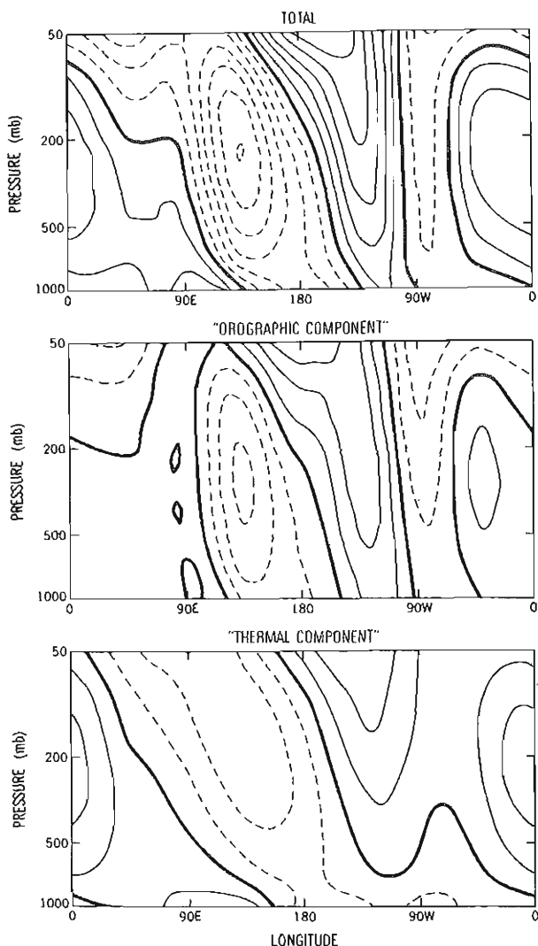
Fig. 6.20. The eddy geopotential height as a function of longitude and pressure at 45^{\circ}\text{N} for the mountain model ('total'), the mountain minus no-mountain flow ('orographic component') and the no-mountain model ('thermal component'). The contour interval is 50 m with negative contours dashed. Model fields in Figs. 6.19–6.23 are averaged over the three winter months in each of the 15 model years.
