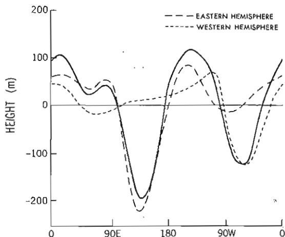
Fig. 6.3. The response shown in Fig. 6.2 split into the parts due to the topography of the western and eastern hemispheres.
