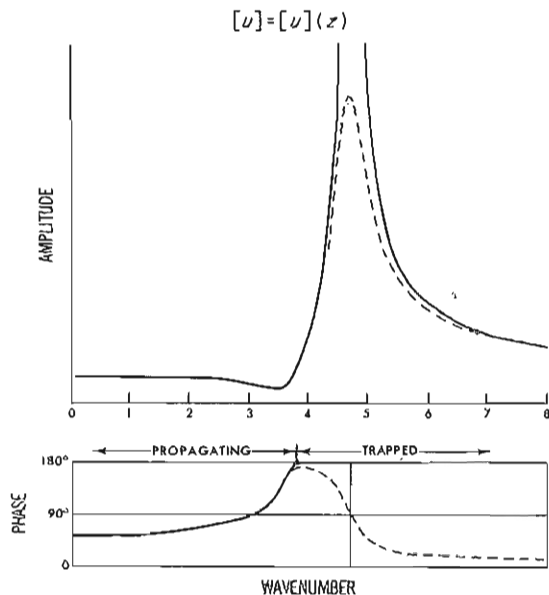
Fig. 6.16. Same as Fig. 6.13 for the wind profile shown in Fig. 6.14.
