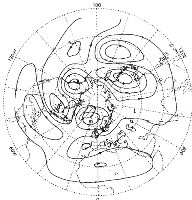
Fig. 6.23. The streamfunction for the mountain minus no-mountain flow at 300 mb. Contour interval is 4 \times 10^6 \text{ m}^2 \text{ s}^{-1} .
