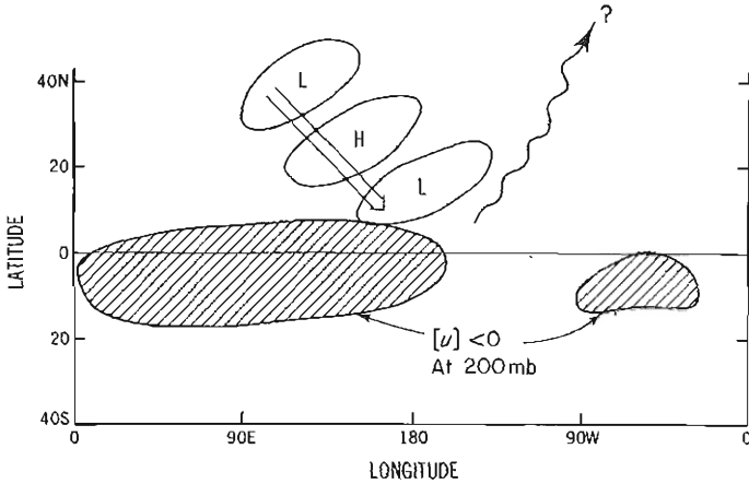
Fig. 6.11. Schematic of the Rossby wavetrain generated by the Tibetan plateau propagating into the tropics.
