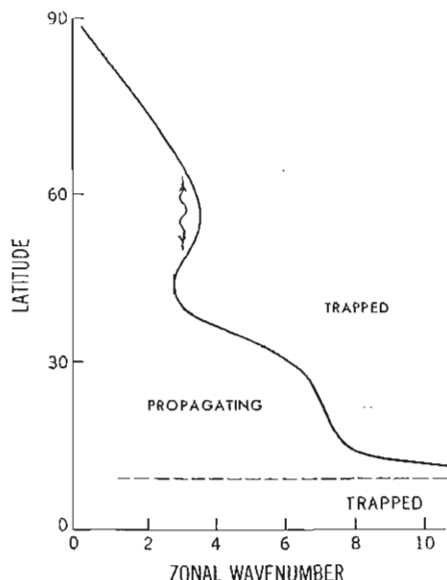
Fig. 6.10. The wavenumber, n_s = ak_s , dividing propagating from evanescent solutions for a mean wind resembling the wintertime flow at 300 mb, from Karoly (1978). The arrows indicate the potential for meridional confinement of wavenumber 3 near 55°.
