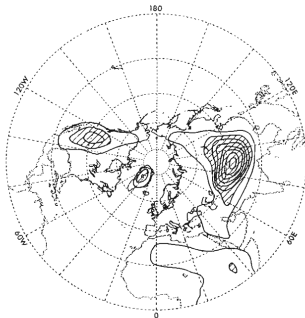
Fig. 6.5. The topography used in the spherical barotropic calculations, taken from the low resolution spectral model described in Section 6.6. The contour interval is 500 m and heights over 1 km are shaded. The zero contour is not shown. The concentric dotted circles are 20^\circ latitude apart, the outer circle being the equator.
