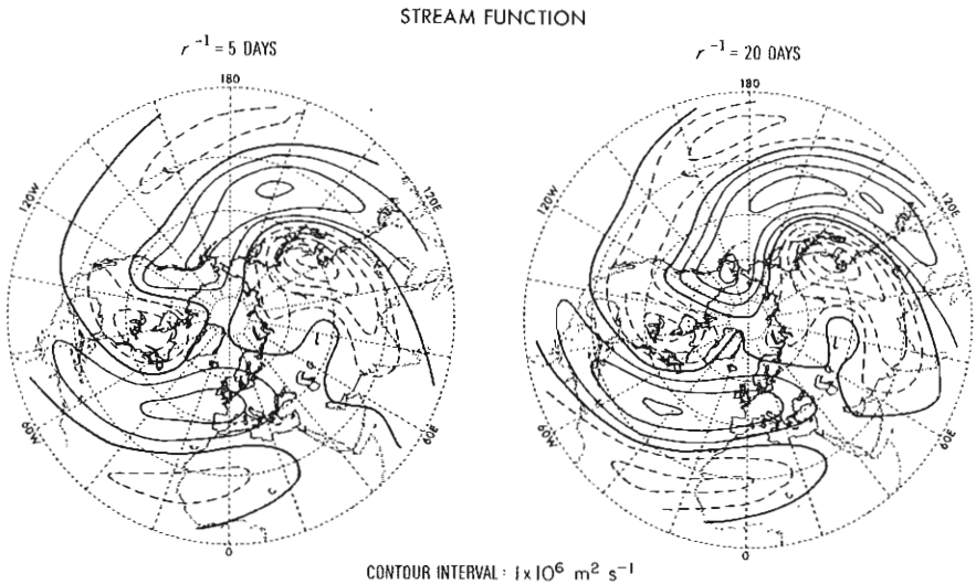
Fig. 6.7. The streamfunction response in the Northern Hemisphere of the barotropic model, using the topography and mean winds in Figs. 6.5 and 6.6, for two different levels of dissipation. Solid contours are positive or zero; dotted contours are negative.
